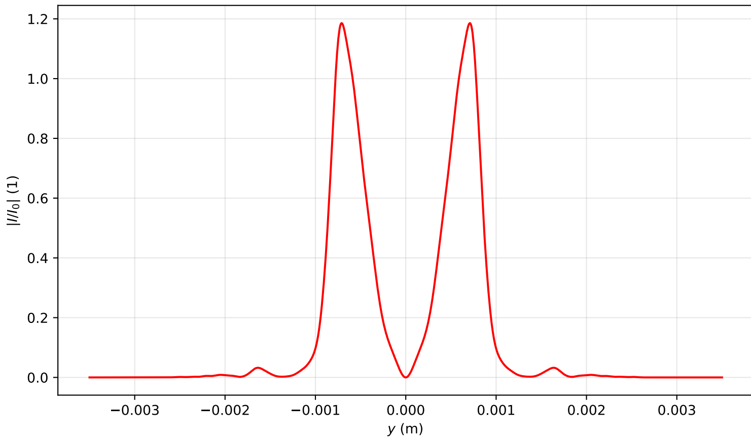
Intensity profile I(x=0, y, z=1.353)/I_0 , P_{in}=13.0P_{cr} , artificial time
