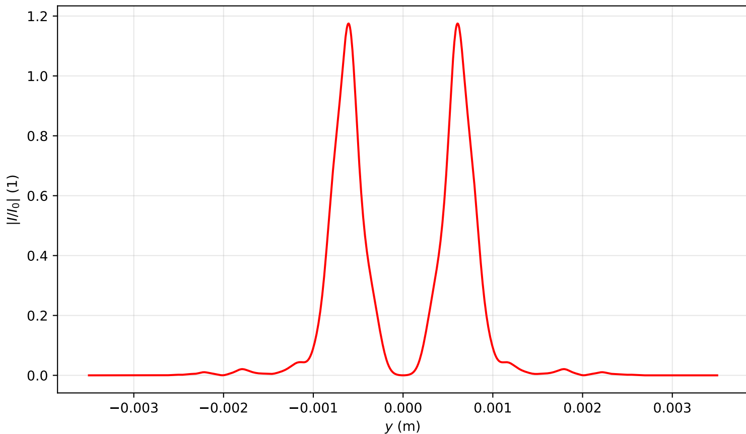
Intensity profile I(x=0, y, z=1.433)/I_0 , P_{in}=13.0P_{cr} , artificial time
