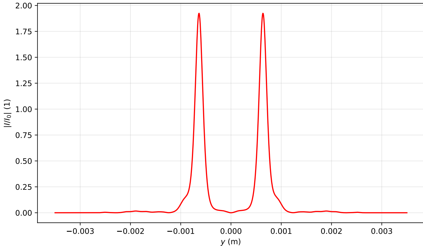
Intensity profile I(x=0, y, z=1.592)/I_0 , P_{in}=13.0P_{cr} , artificial time
