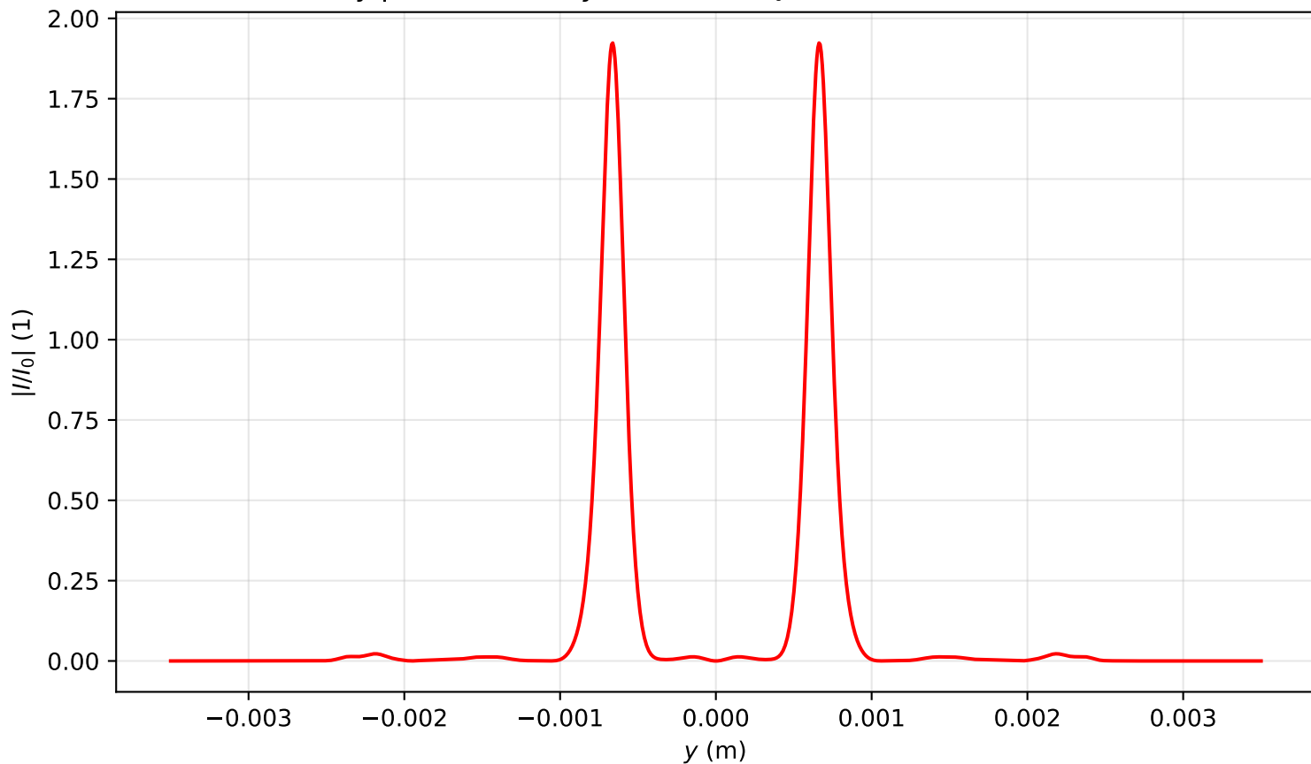
Intensity profile I(x=0, y, z=1.751)/I_0 , P_{in}=13.0P_{cr} , artificial time
