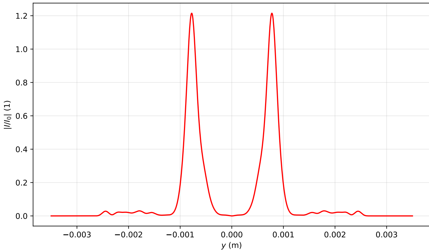
Intensity profile I(x=0, y, z=2.388)/I_0 , P_{in}=13.0P_{cr} , artificial time
