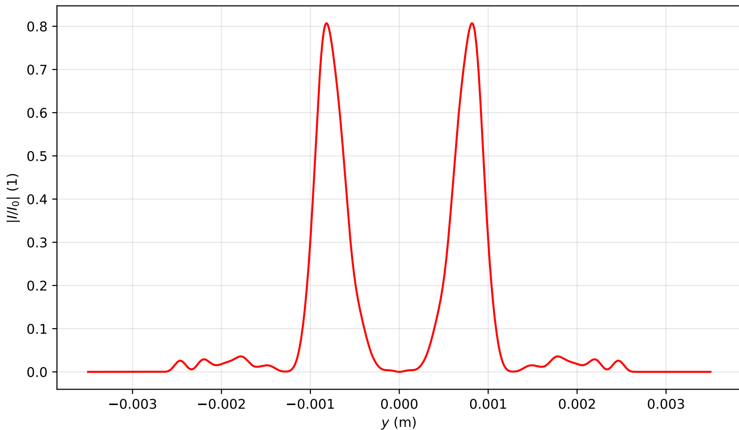
Intensity profile I(x=0, y, z=2.468)/I_0 , P_{in}=13.0\text{Pcr} , artificial time
