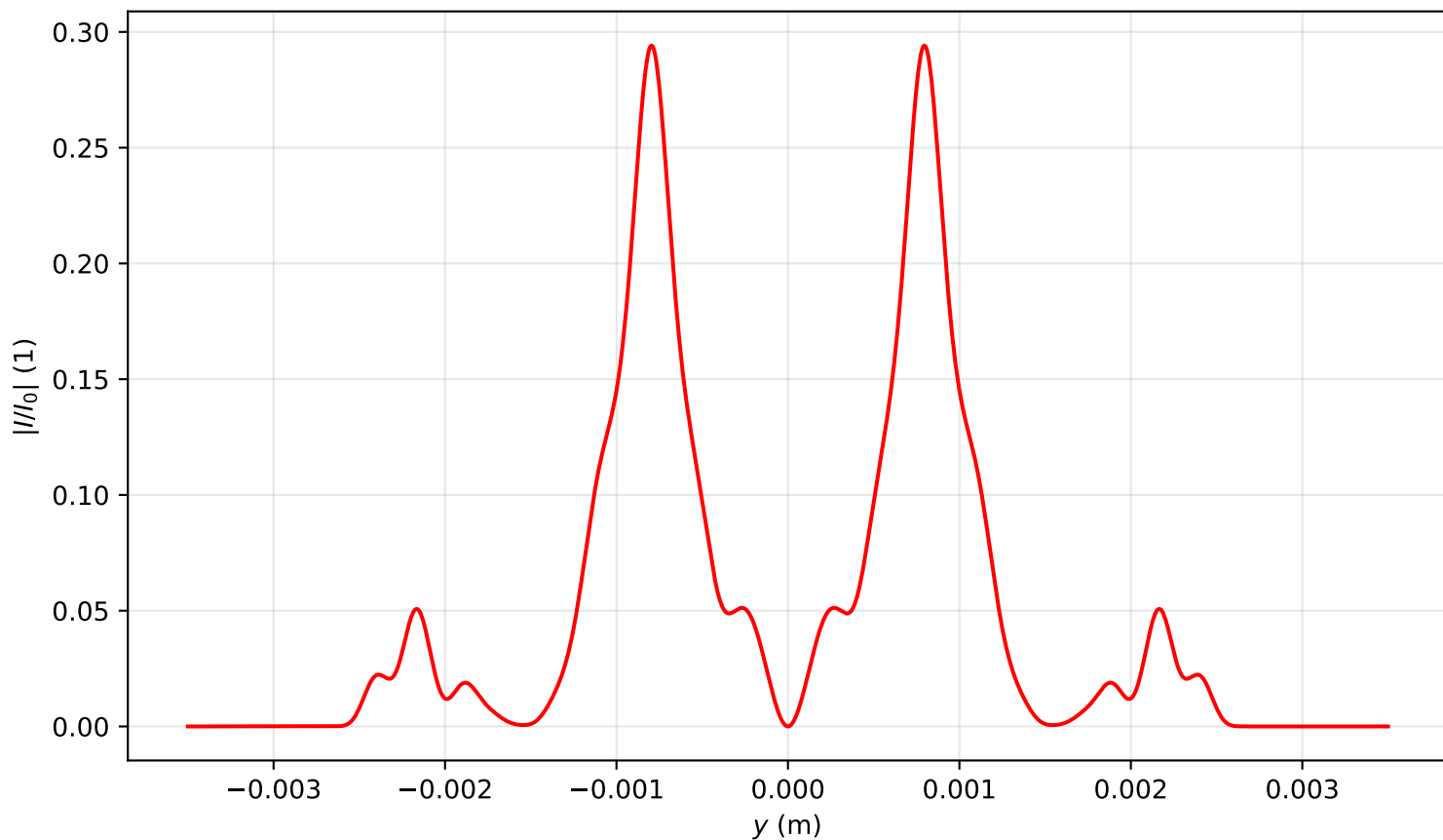
Intensity profile I(x = 0, y, z = 2.786)/I_0 , P_{in}=13.0P_{cr} , artificial time
