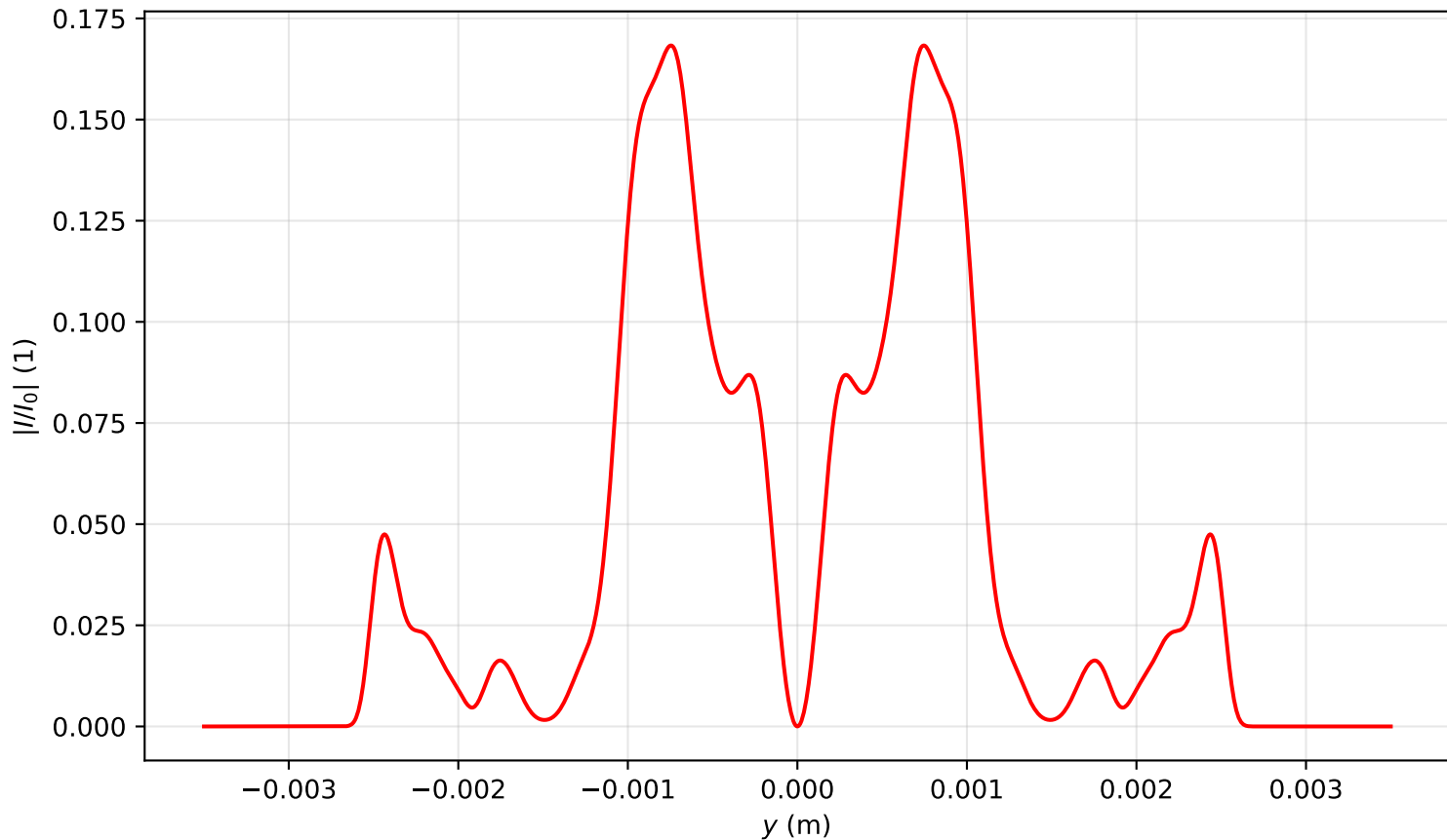
Intensity profile I(x=0, y, z=2.946)/I_0 , P_{in}=13.0P_{cr} , artificial time
