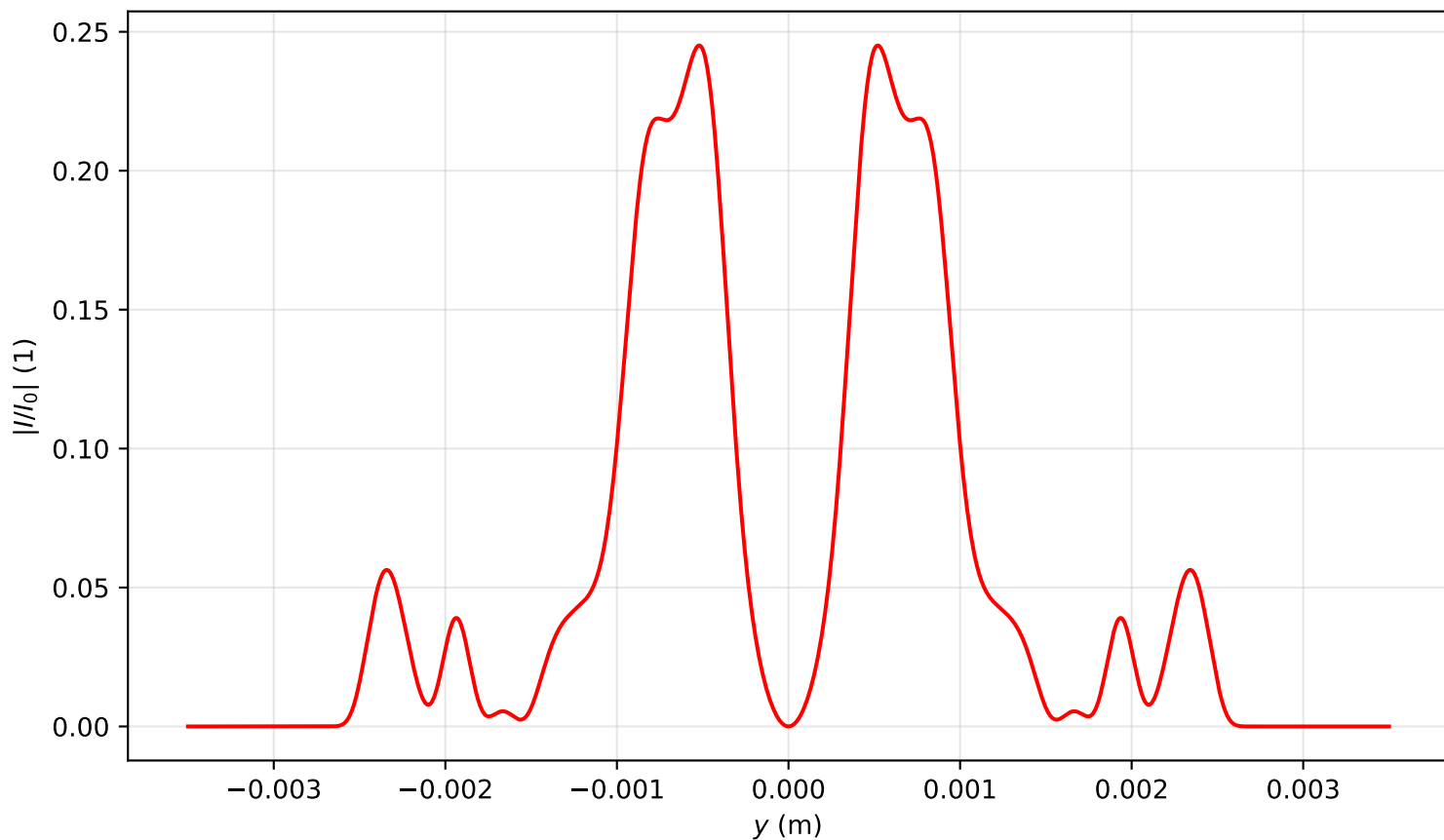
Intensity profile I(x = 0, y, z = 3.423)/I_0 , P_{in}=13.0P_{cr} , artificial time
