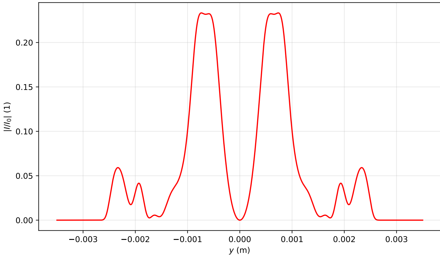
Intensity profile I(x=0, y, z=3.503)/I_0 , P_{in}=13.0P_{cr} , artificial time
