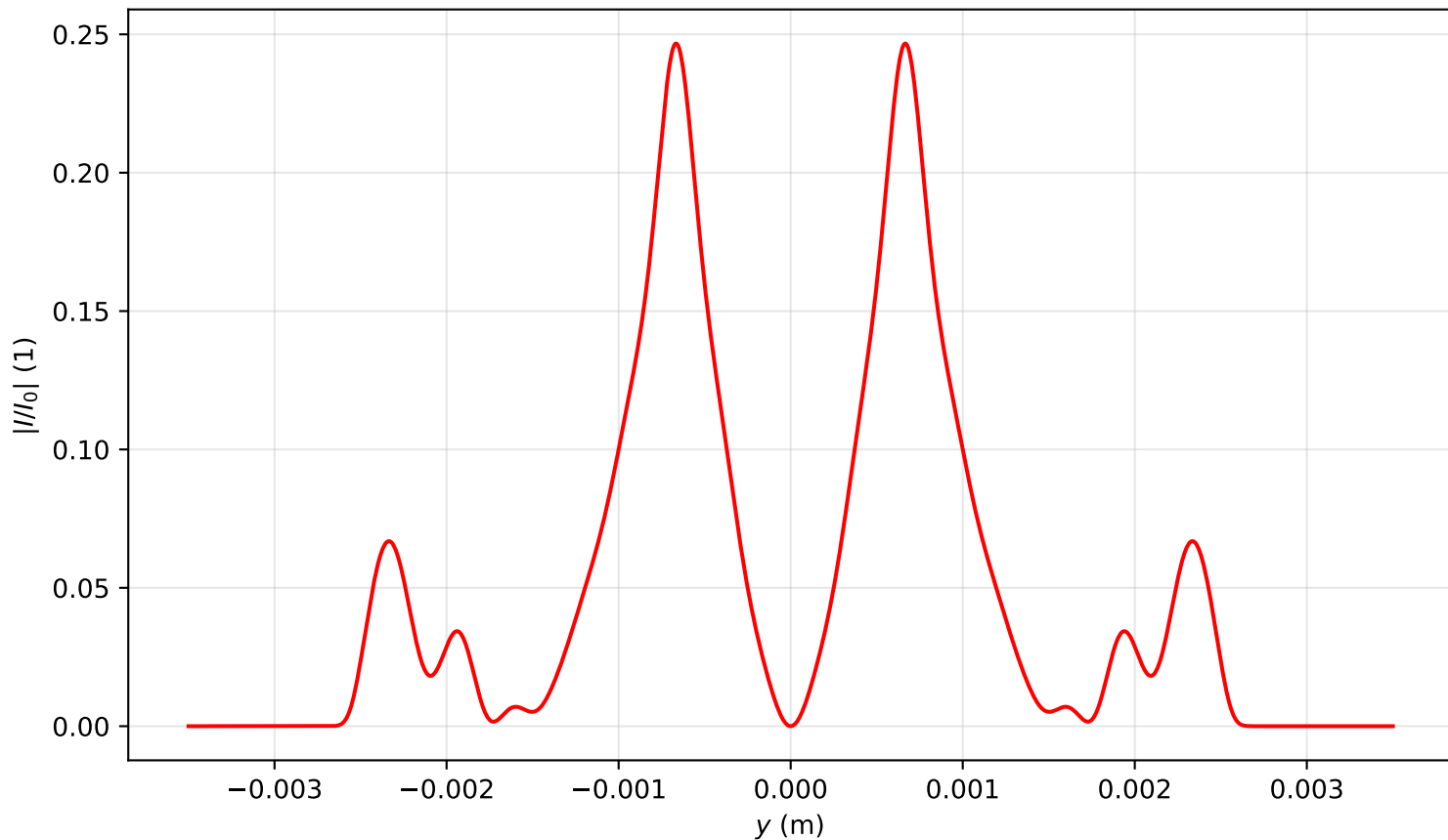
Intensity profile I(x=0, y, z=3.582)/I_0 , P_{in}=13.0P_{cr} , artificial time
