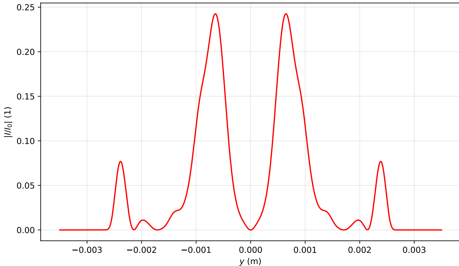
Intensity profile I(x=0, y, z=3.901)/I_0 , P_{in}=13.0P_{cr} , artificial time
