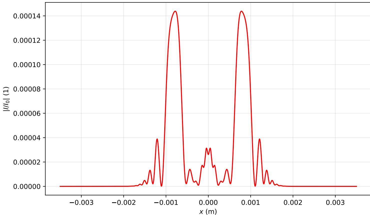
Intensity profile I(x, y = 0, z = 0.398)/I_0 , P_{in}=14.0P_{cr} , artificial time
