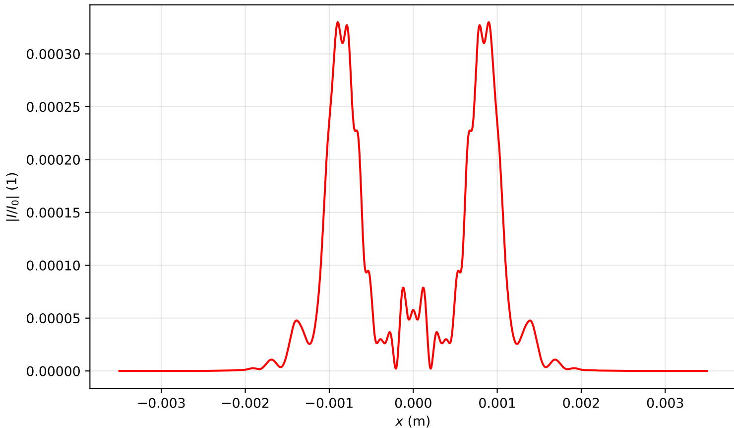
Intensity profile I(x, y = 0, z = 0.557)/I_0 , P_{in}=14.0P_{cr} , artificial time
