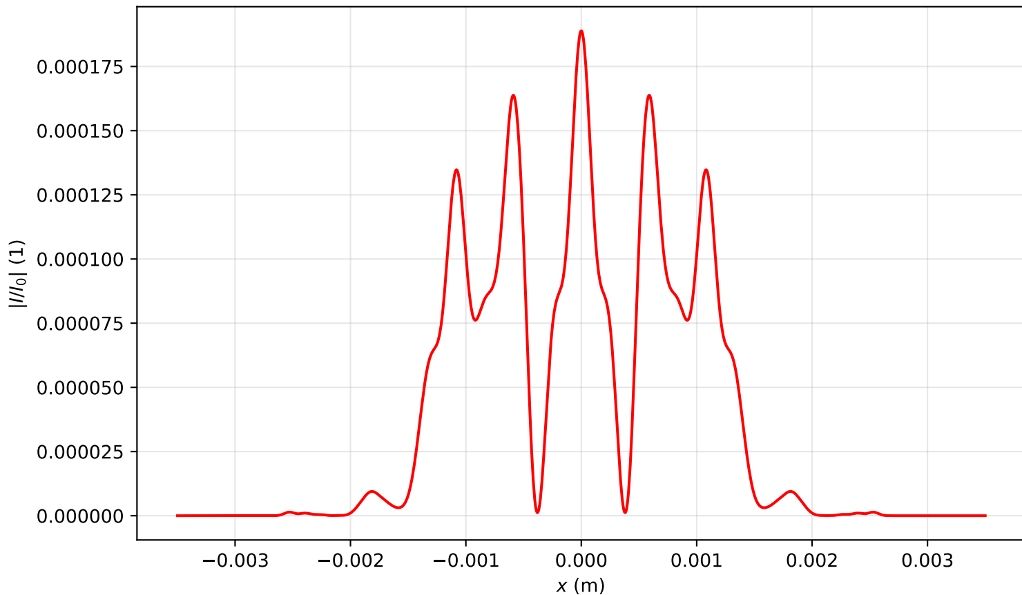
Intensity profile I(x, y = 0, z = 1.035)/I_0 , P_{in}=14.0P_{cr} , artificial time
