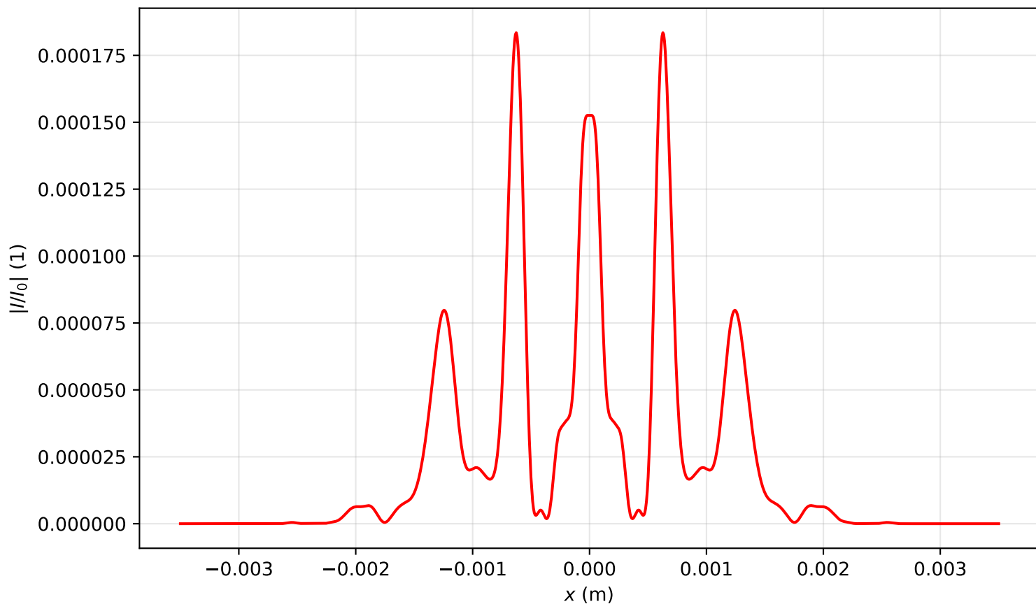
Intensity profile I(x, y = 0, z = 1.115)/I_0 , P_{in}=14.0\text{Pcr} , artificial time
