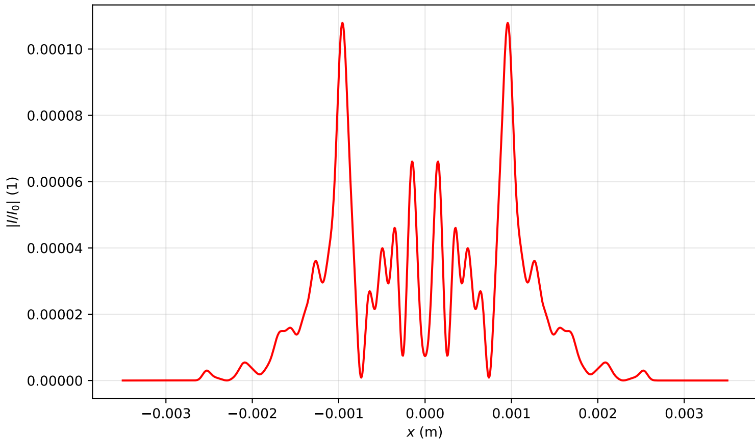
Intensity profile I(x, y = 0, z = 1.353)/I_0 , P_{in}=14.0P_{cr} , artificial time
