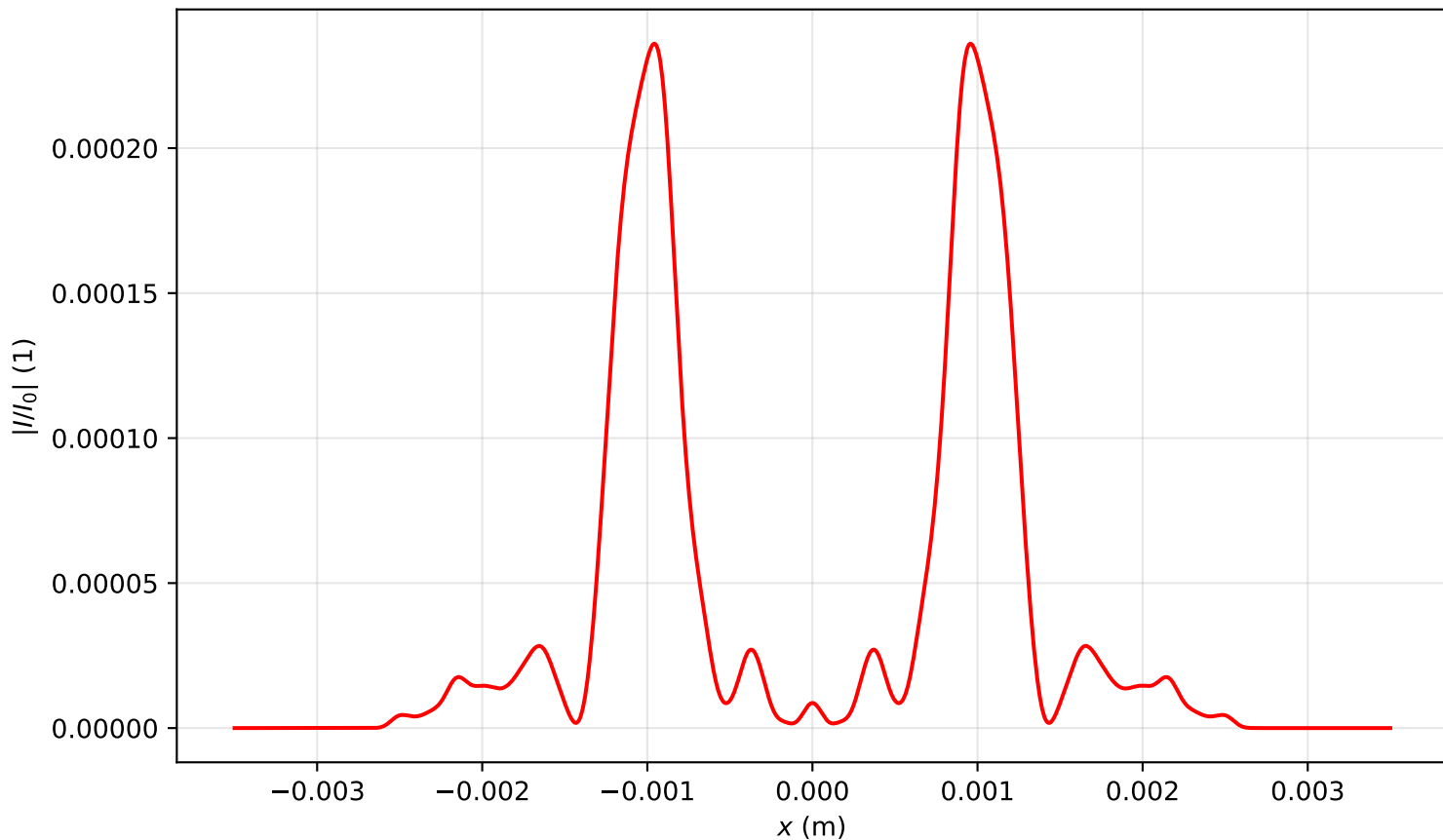
Intensity profile I(x, y = 0, z = 1.831)/I_0 , P_{in}=14.0P_{cr} , artificial time
