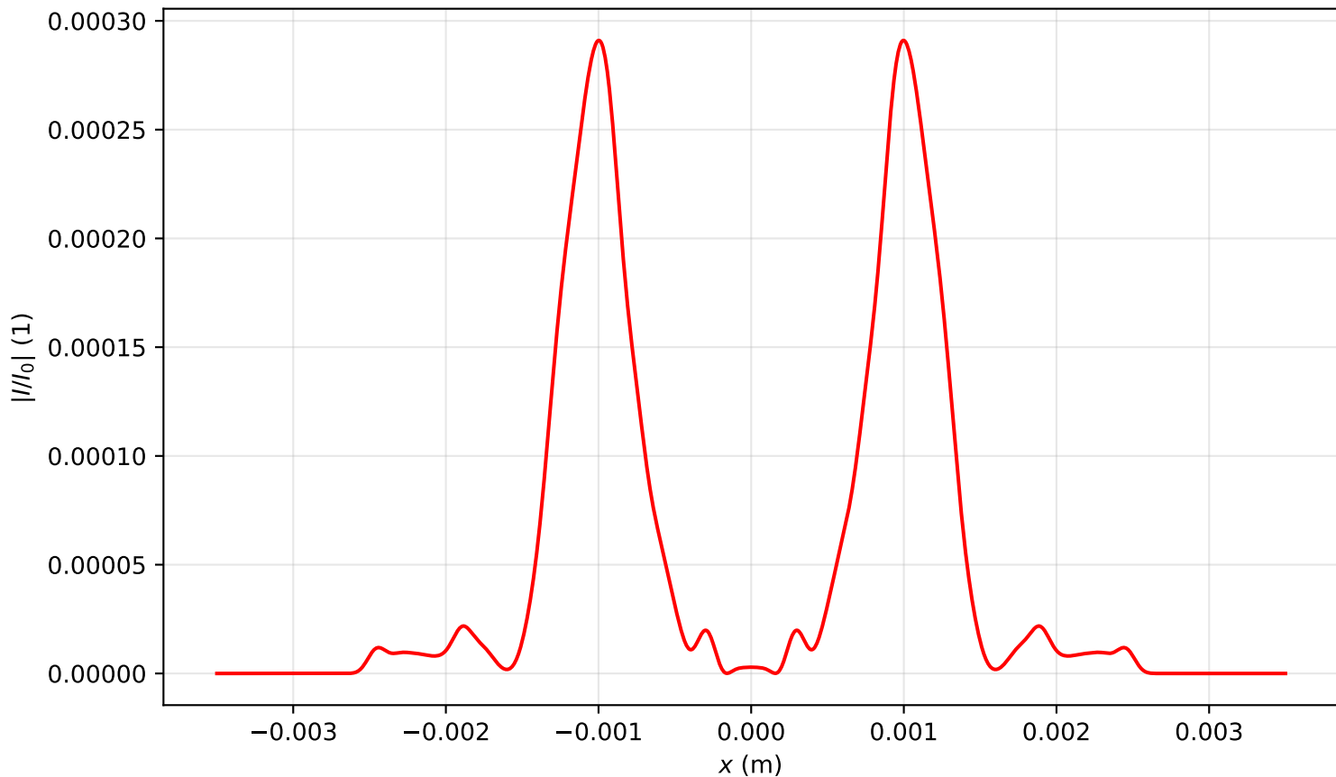
Intensity profile I(x, y = 0, z = 1.911)/I_0 , P_{in}=14.0\text{Pcr} , artificial time
