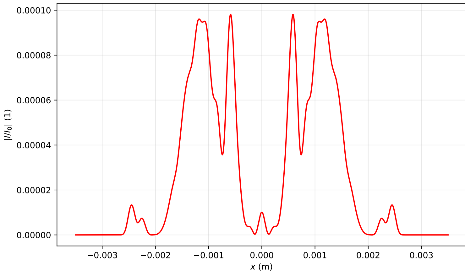
Intensity profile I(x, y = 0, z = 2.149)/I_0 , P_{in}=14.0P_{cr} , artificial time
