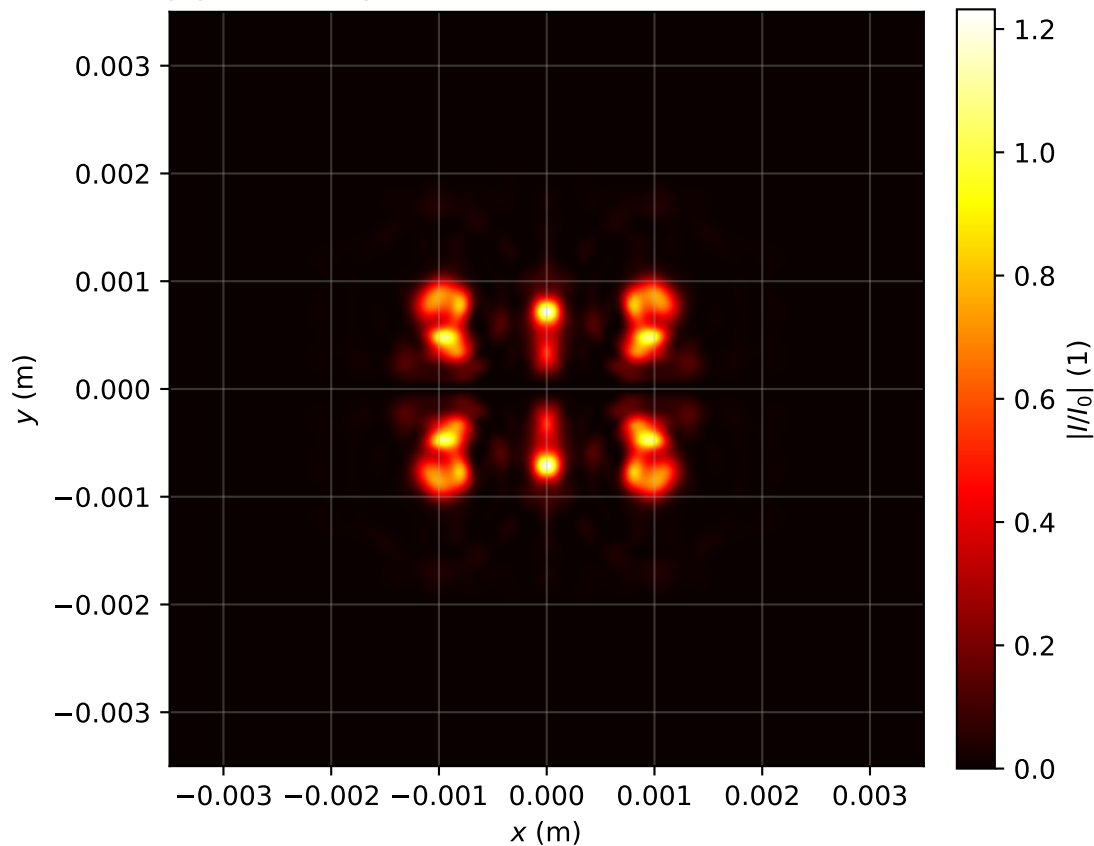
Intensity profile I(x, y, z = 1.194)/I_0 , P_{in}=14.0\text{Pcr} , artificial time
