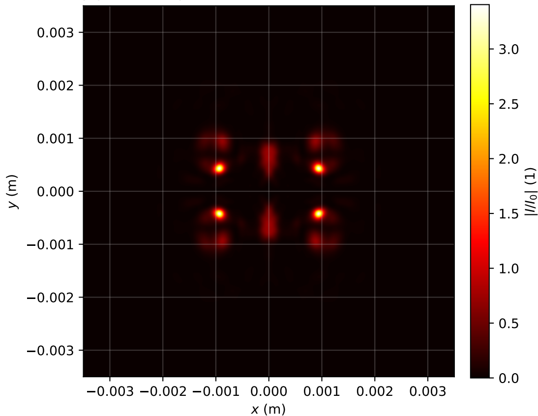
Intensity profile I(x, y, z = 1.353)/I_0 , P_{in}=14.0\text{Pcr} , artificial time
