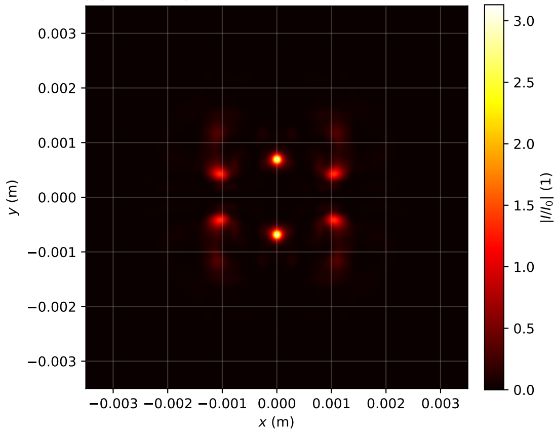
Intensity profile I(x, y, z = 1.751)/I_0 , P_{in}=14.0\text{Pcr} , artificial time
