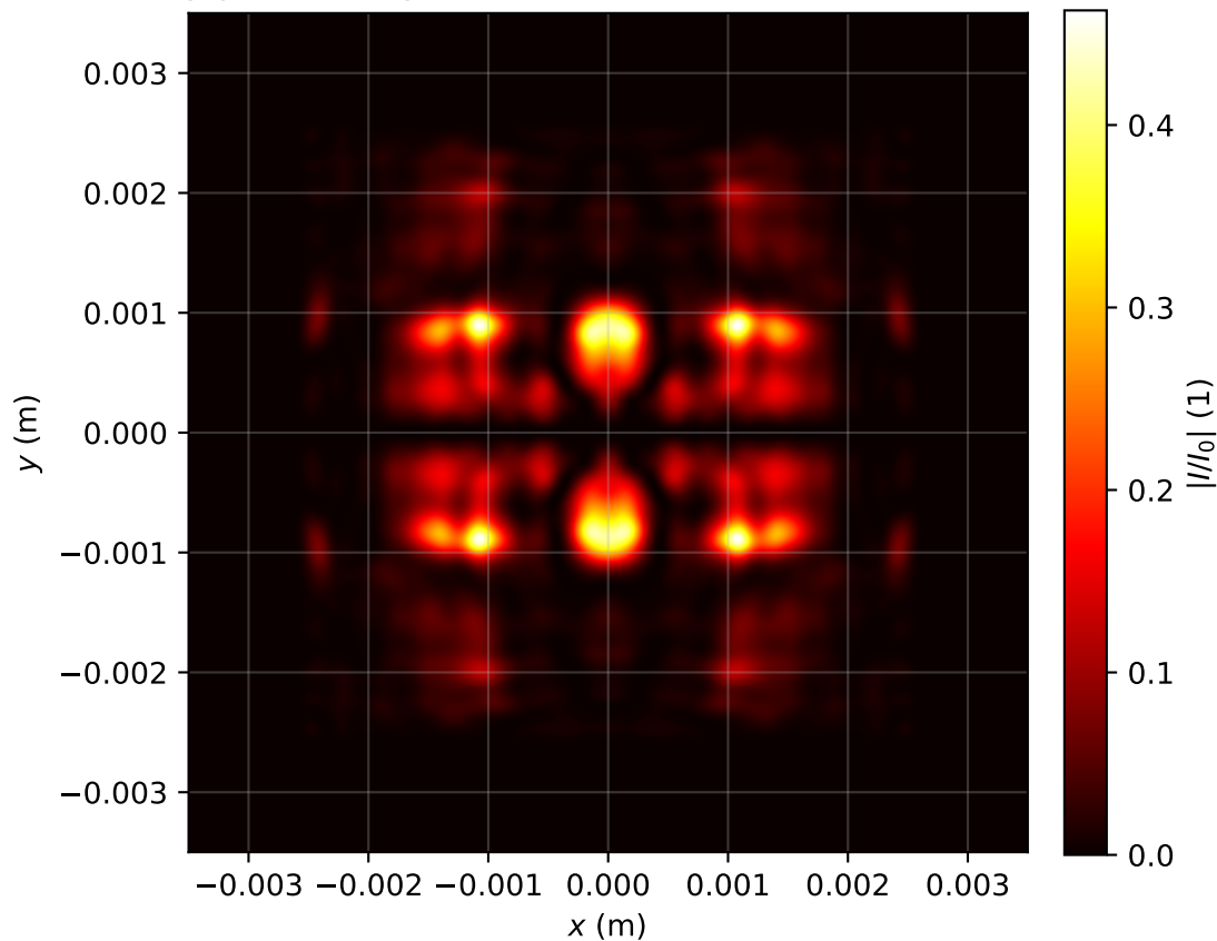
Intensity profile I(x, y, z = 2.309)/I_0 , P_{in}=14.0\text{Pcr} , artificial time
