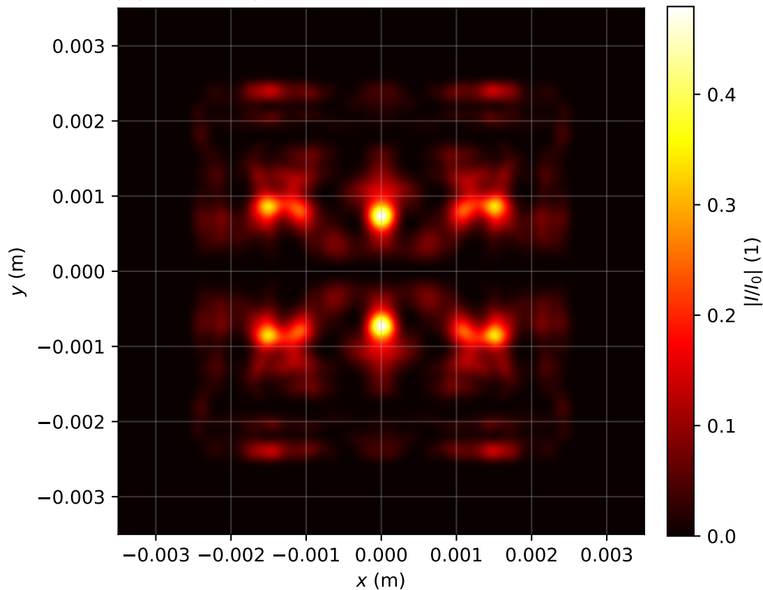
Intensity profile I(x, y, z = 2.946)/I_0 , P_{in}=14.0\text{Pcr} , artificial time
