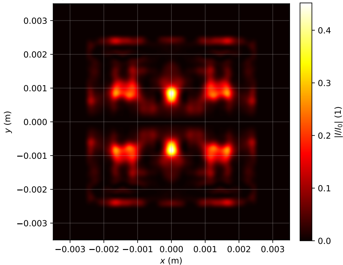
Intensity profile I(x, y, z = 3.105)/I_0 , P_{in}=14.0\text{Pcr} , artificial time
