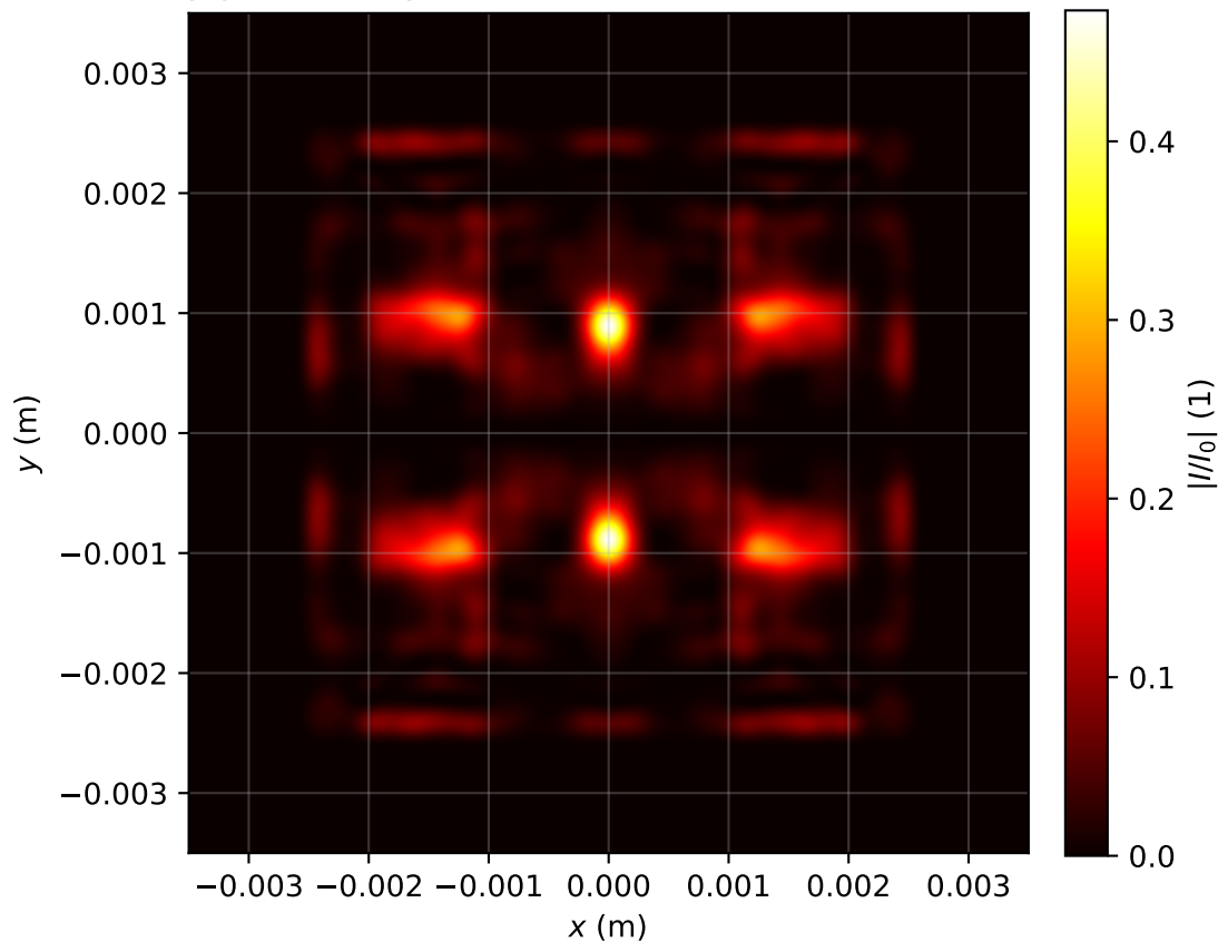
Intensity profile I(x, y, z = 3.264)/I_0 , P_{in}=14.0\text{Pcr} , artificial time
