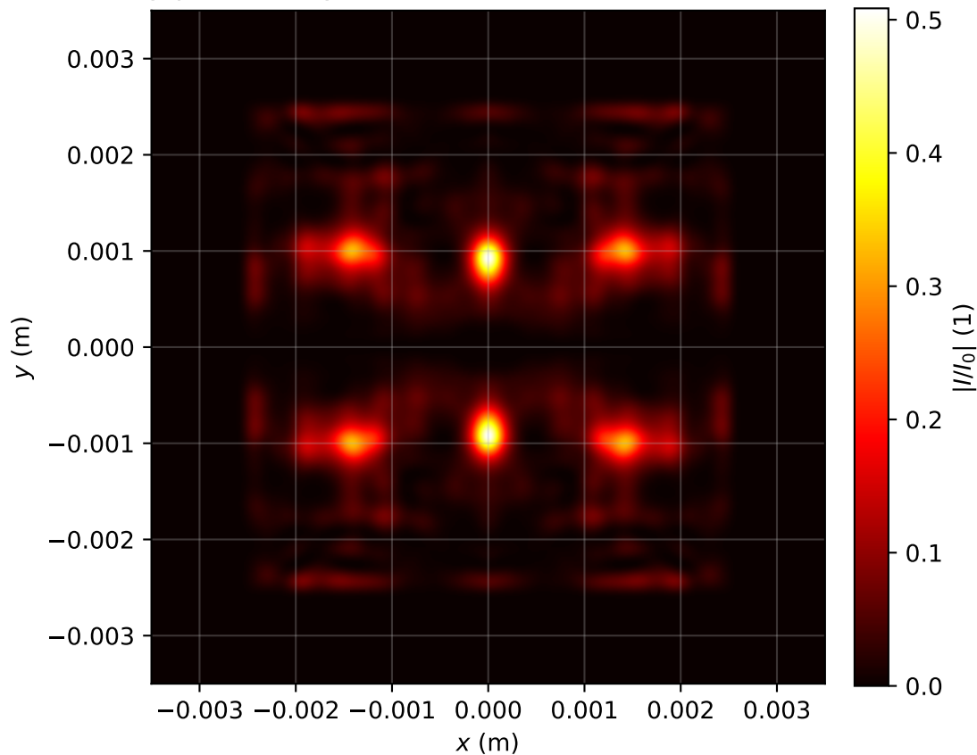
Intensity profile I(x, y, z = 3.344)/I_0 , P_{in}=14.0P_{cr} , artificial time
