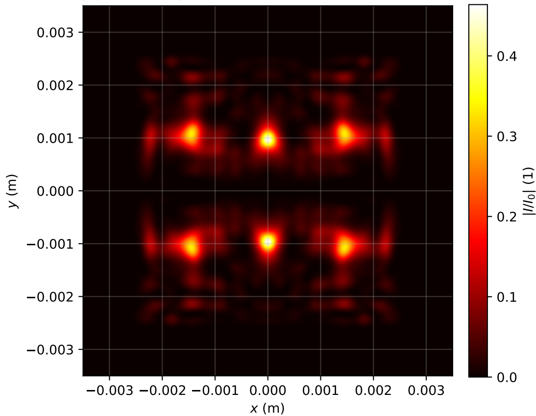
Intensity profile I(x, y, z = 3.582)/I_0 , P_{in}=14.0\text{Pcr} , artificial time
