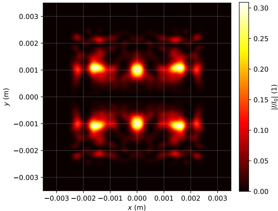
Intensity profile I(x, y, z = 3.742)/I_0 , P_{in}=14.0P_{cr} , artificial time
