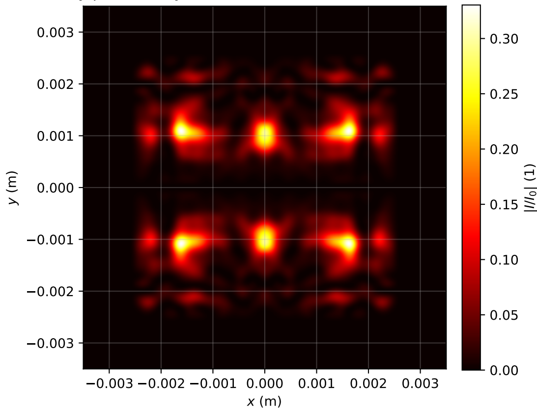
Intensity profile I(x, y, z = 3.821)/I_0 , P_{in}=14.0\text{Pcr} , artificial time
