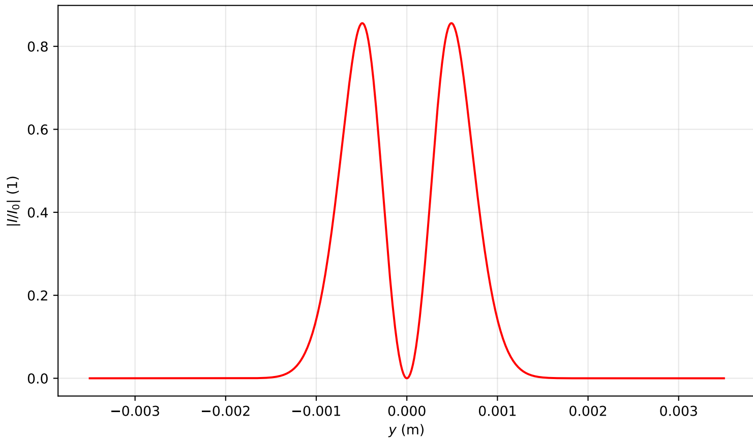
Intensity profile I(x=0, y, z=0.080)/I_0 , P_{in}=14.0P_{cr} , artificial time
