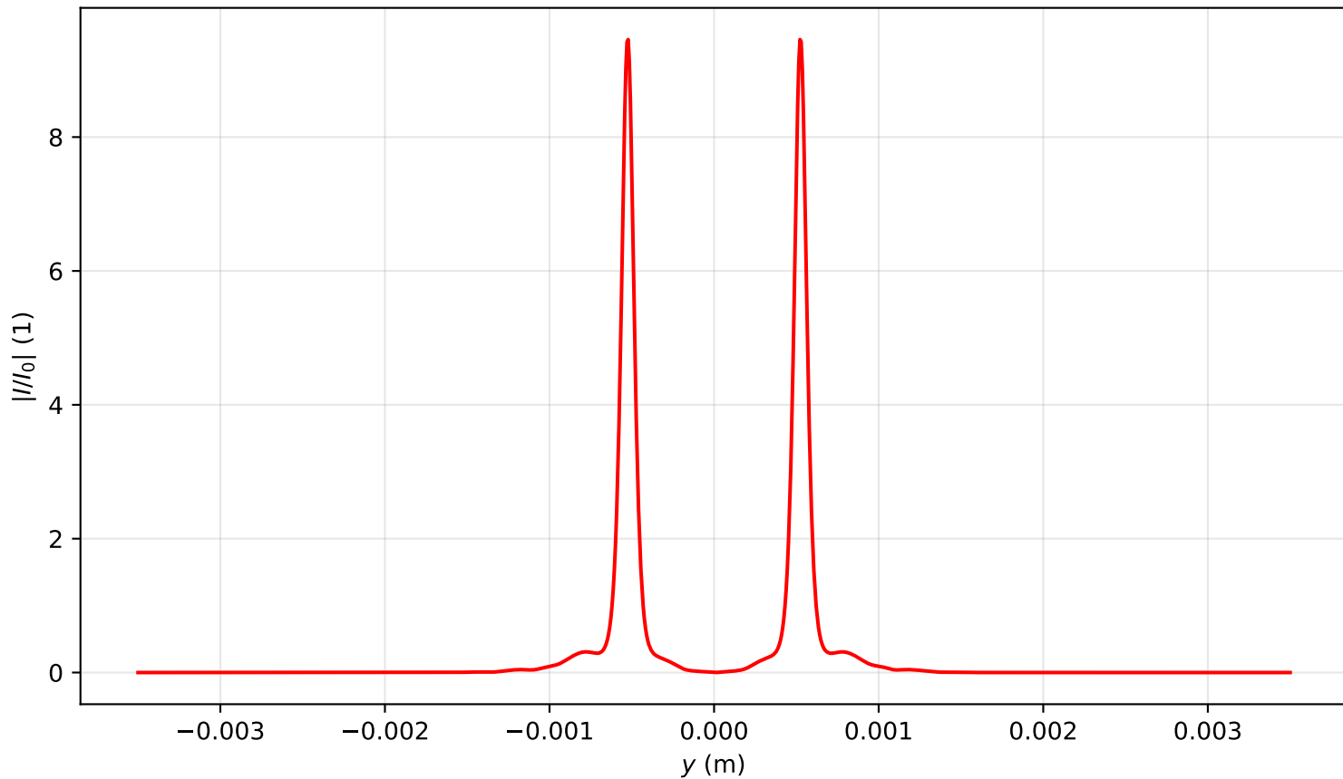
Intensity profile I(x=0, y, z=0.557)/I_0 , P_{in}=14.0\text{Pcr} , artificial time
