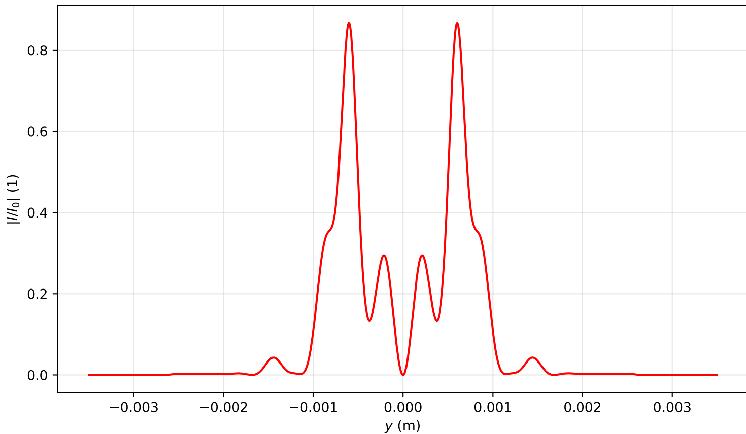
Intensity profile I(x=0, y, z=1.035)/I_0 , P_{in}=14.0P_{cr} , artificial time
