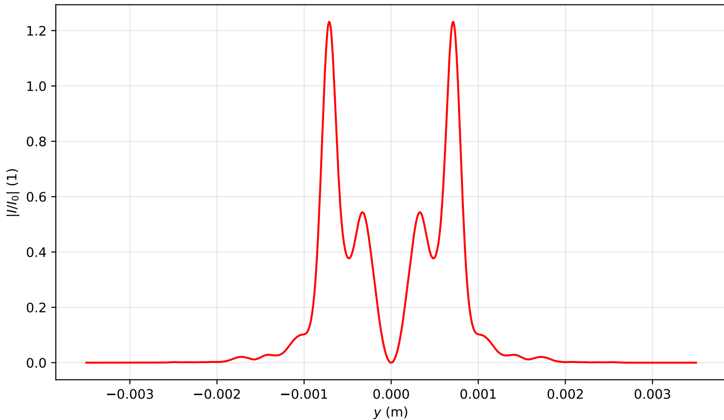
Intensity profile I(x=0, y, z=1.194)/I_0 , P_{in}=14.0\text{Pcr} , artificial time
