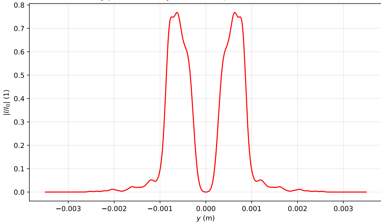
Intensity profile I(x=0, y, z=1.353)/I_0 , P_{in}=14.0P_{cr} , artificial time
