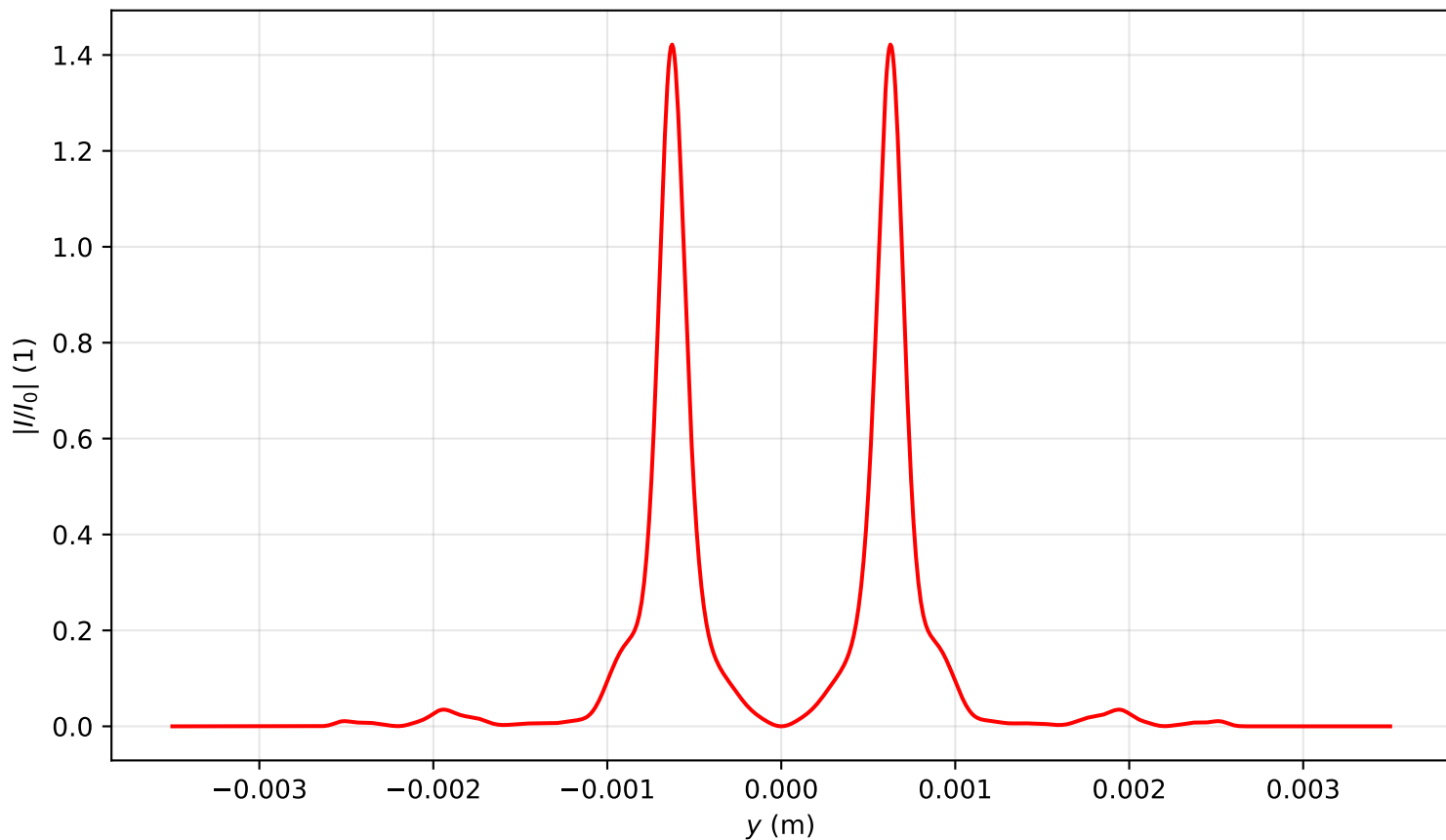
Intensity profile I(x=0, y, z=1.513)/I_0 , P_{in}=14.0\text{Pcr} , artificial time
