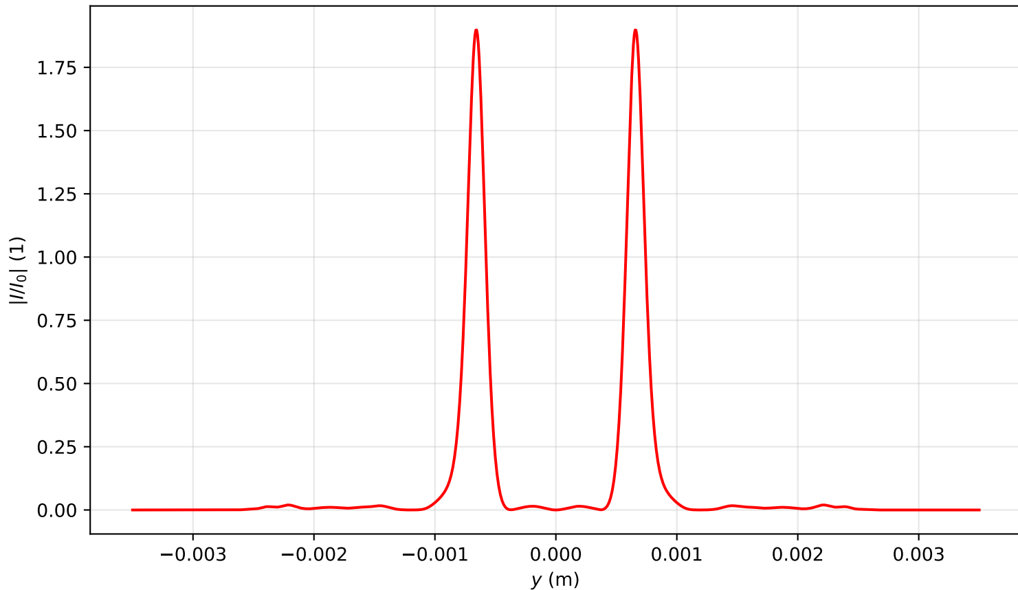
Intensity profile I(x=0, y, z=1.672)/I_0 , P_{in}=14.0P_{cr} , artificial time
