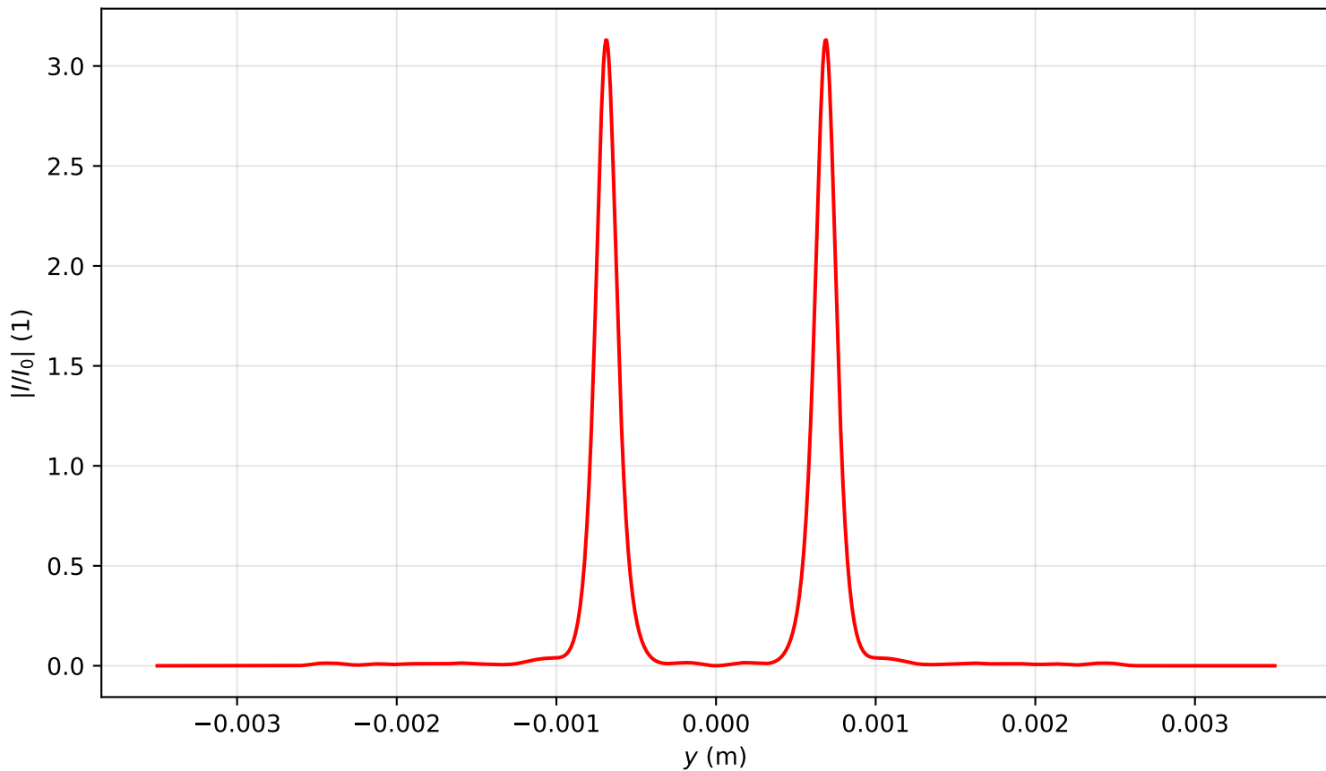
Intensity profile I(x=0, y, z=1.751)/I_0 , P_{in}=14.0P_{cr} , artificial time
