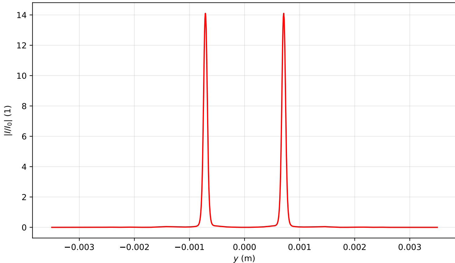
Intensity profile I(x = 0, y, z = 1.911)/I_0 , P_{in}=14.0\text{Pcr} , artificial time
