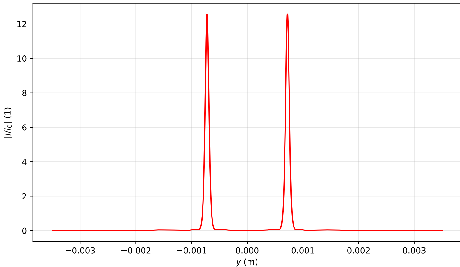
Intensity profile I(x = 0, y, z = 1.990)/I_0 , Pin=14.0Pcr, artificial time
