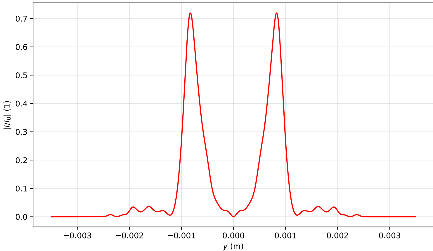
Intensity profile I(x=0, y, z=2.229)/I_0 , P_{in}=14.0\text{Pcr} , artificial time
