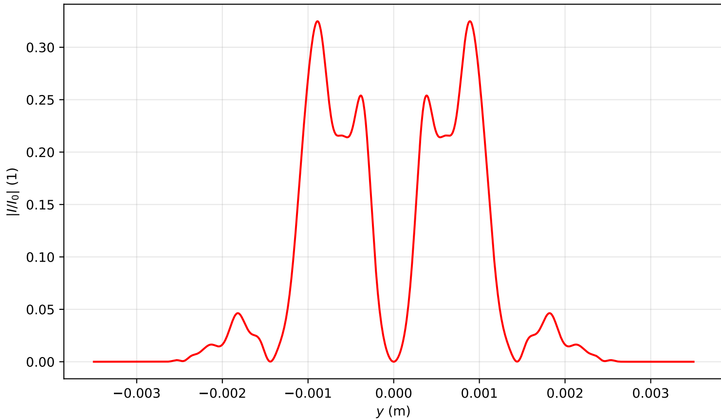
Intensity profile I(x=0, y, z=2.468)/I_0 , P_{in}=14.0\text{Pcr} , artificial time
