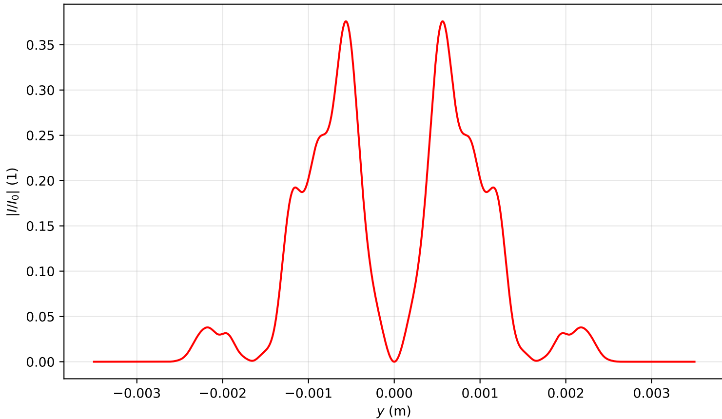
Intensity profile I(x = 0, y, z = 2.707)/I_0 , P_{in}=14.0P_{cr} , artificial time
