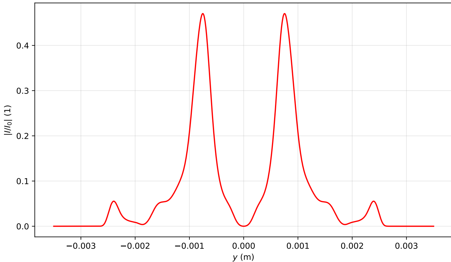
Intensity profile I(x=0, y, z=3.025)/I_0 , P_{in}=14.0P_{cr} , artificial time
