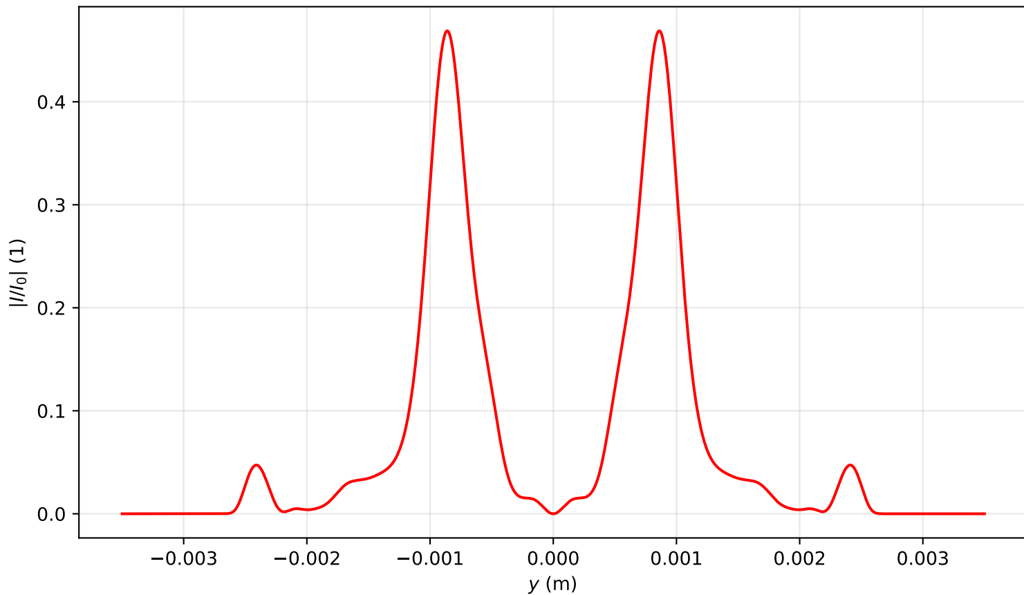
Intensity profile I(x=0, y, z=3.184)/I_0 , P_{in}=14.0P_{cr} , artificial time
