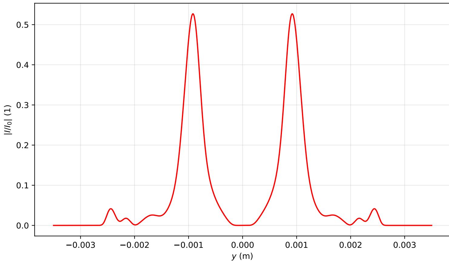
Intensity profile I(x=0, y, z=3.423)/I_0 , P_{in}=14.0\text{Pcr} , artificial time
