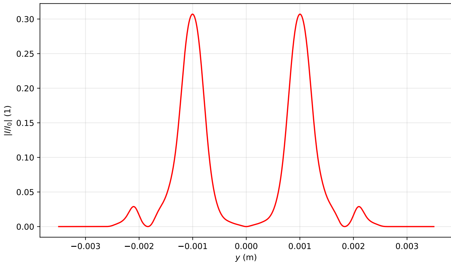
Intensity profile I(x=0, y, z=3.901)/I_0 , P_{in}=14.0\text{Pcr} , artificial time
