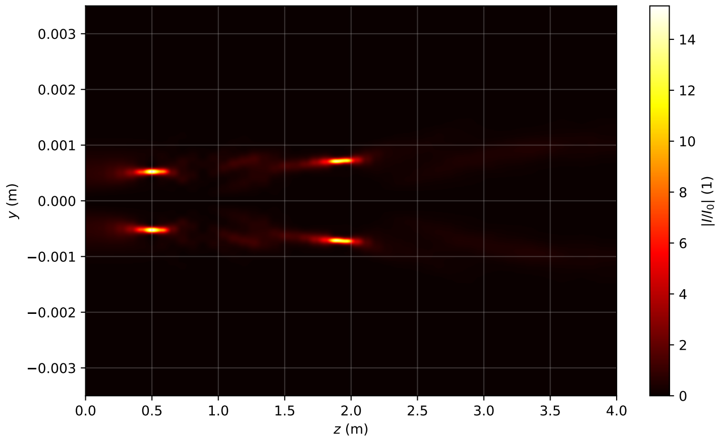
Intensity profile I(x = 0, y, z)/I_0 , P_{in}=14.0P_{cr} , artificial time
