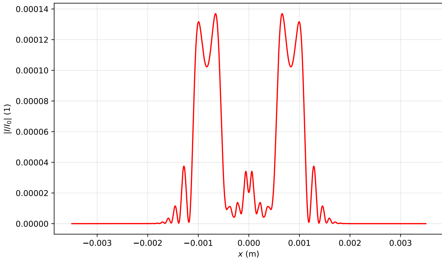
Intensity profile I(x, y = 0, z = 0.398)/I_0 , P_{in}=15.0P_{cr} , artificial time
